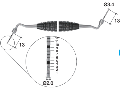
Depth Gauge
