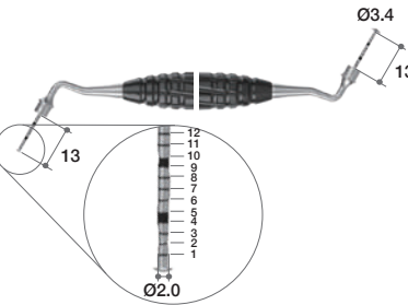
Depth Gauge
